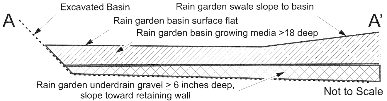
Figure 2A: Section A-A' Schematic from Rain Garden Basin NE to Swale
