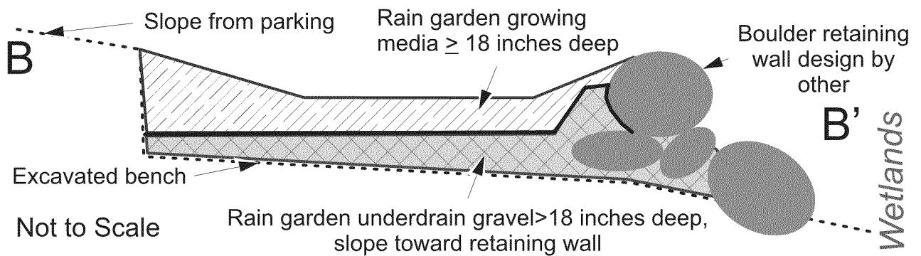
Figure 2B: Section B-B' Schematic across Rain Garden Swale
